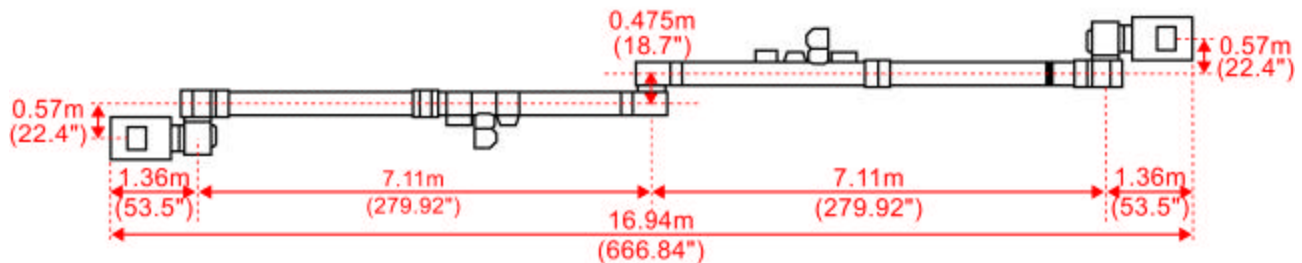
Figure 1: SSRMS Dimensions
