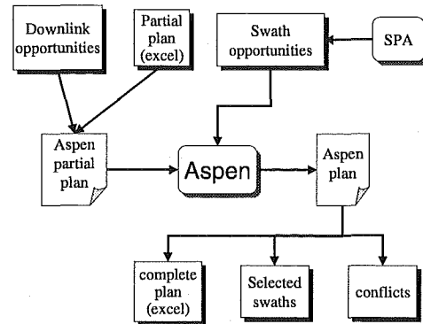
Figure 1: System Data Flow Architecture
