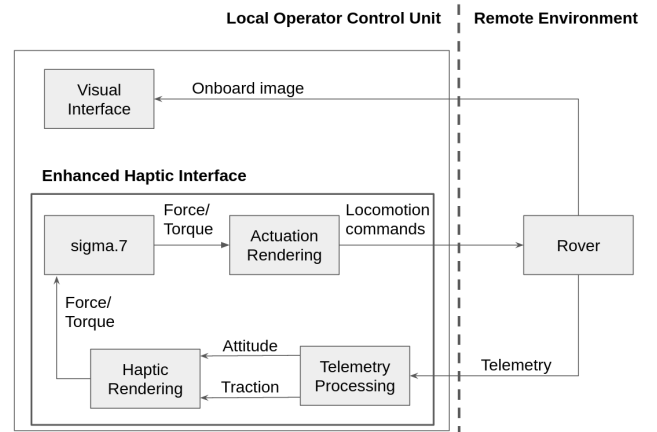
Figure 5. System architecture for the proposed teleoperation interface.
